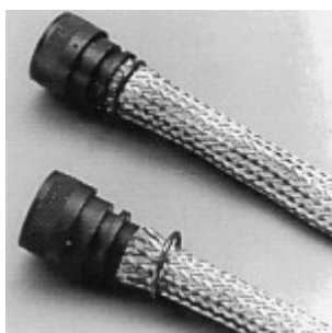
Fig. 12: Electromagnetic shielding braid termination with fastener rings [12]
