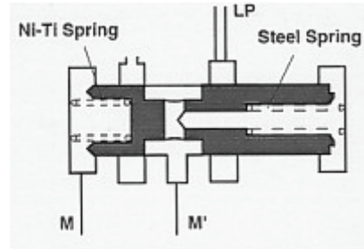
Fig. 19: as 18, function schematic [19]
