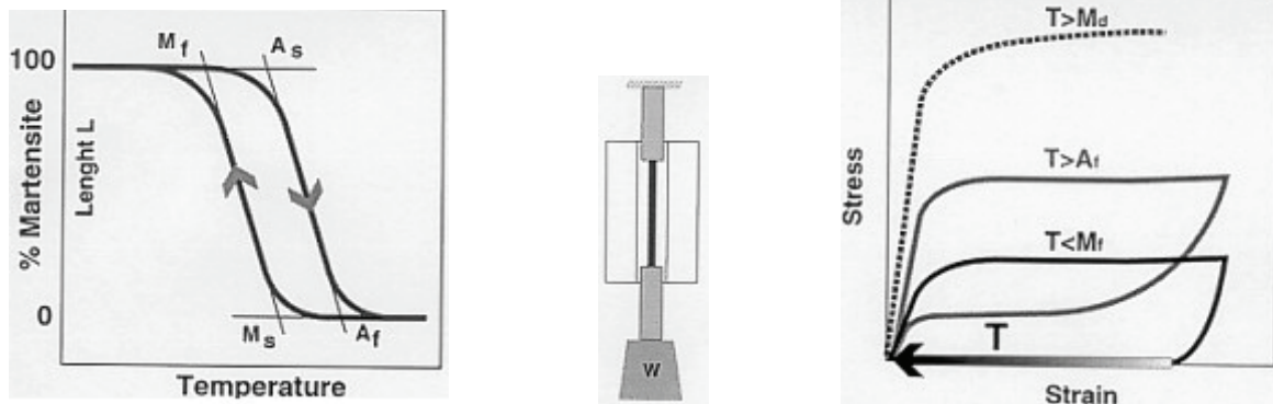
Fig. 2 (left): Schematic representation of the hysteresis loop
