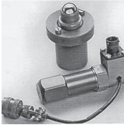
Fig. 24: Clogging indicators for oil coolers [21]
