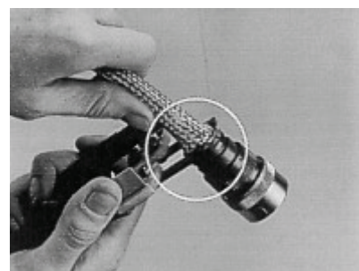
Fig. 13: Installing braid termination rings with conductive heating [12]
