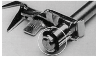
Fig. 15: High amperage pin/socket connector with fastener ring installed [16]
