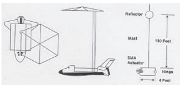
Fig. 28: Active damping system [23]
