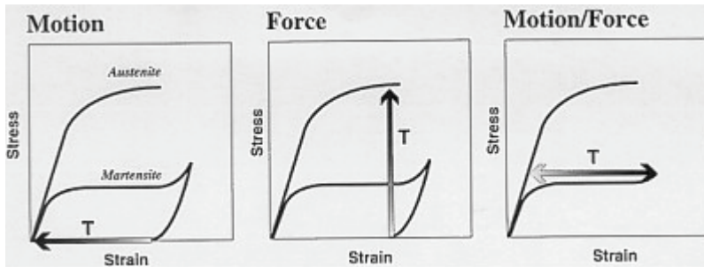
Fig. 6: Shape memory events in the stress/strain perspective [6]
