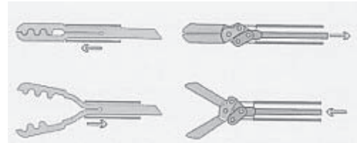
Fig. 33: Hingeless instruments [32]
