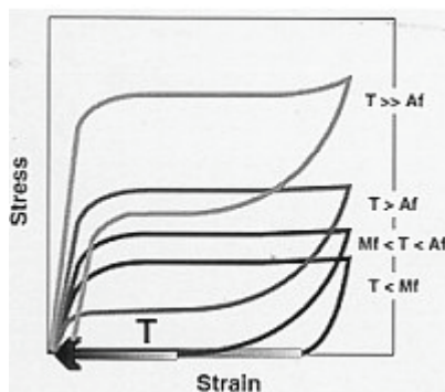
Fig. 8 (left): Tensile behavior of a superelastic wire at different temperatures
