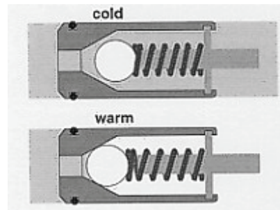
Fig. 23: as 22, schematic function
